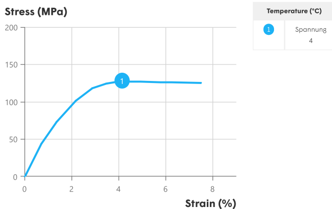
Stress-strain, conditioned
